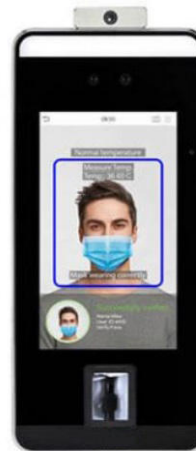
FaceSpeed BioMLV5[TD]
